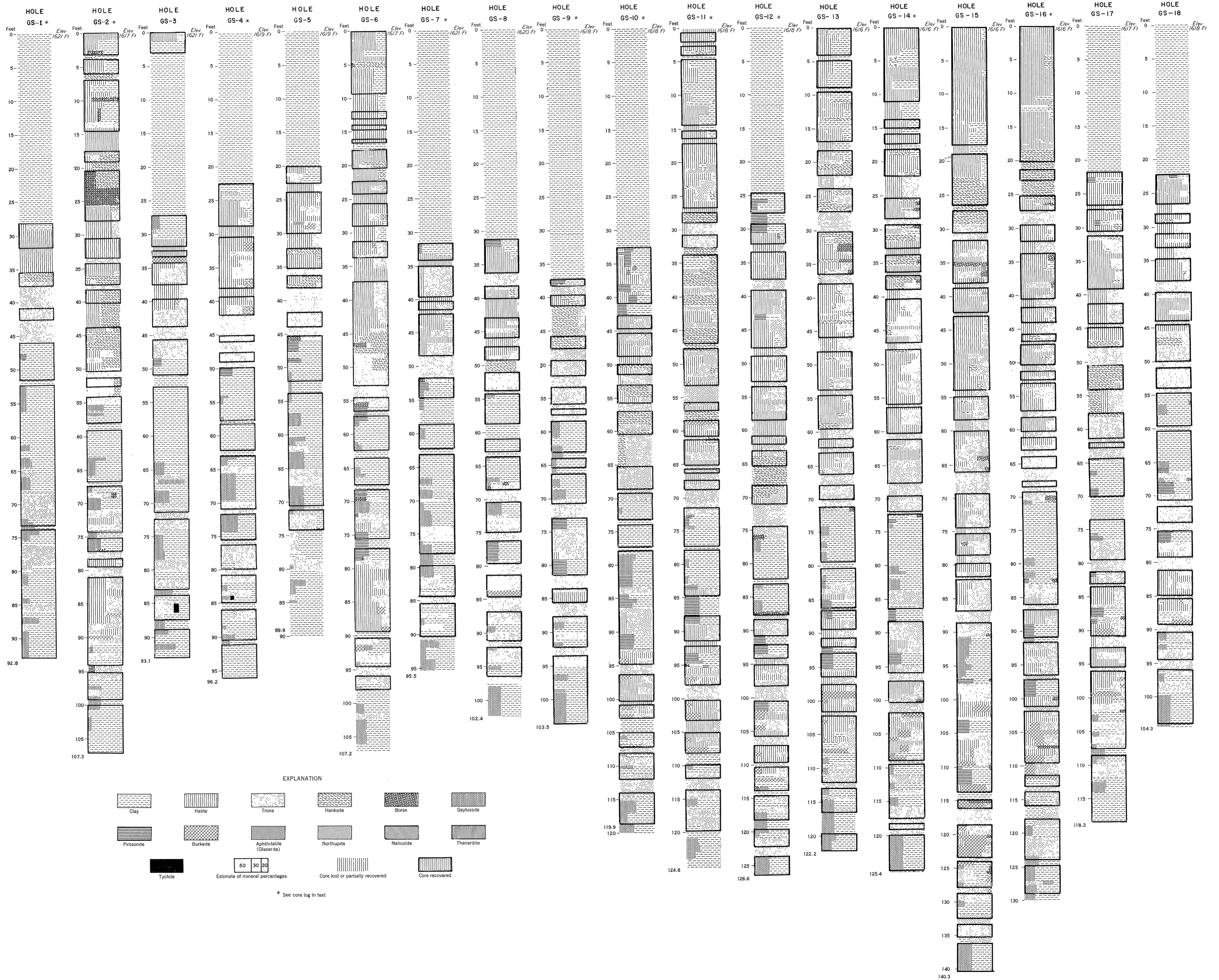
GRAPHIC LOGS OF CORES FROM SEARLES LAKE, CALIFORNIA, DRILL HOLES GS-1 TO GS-18
